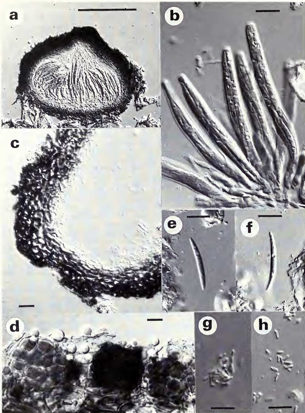
Fig. 42 Cresporhaphis acerina (Rehm) Aguirre (S-lectotype) (a) Vertical section of ascoma; scale = 100 \mu\text{m} ; (b) Asci and ascospores; (c) Detail of exciple: textura angularis; (d) Detail of photobiont and conidiomata; (e), (f) Ascospores; (g) Conidiogenous cell; (h) Conidia; scale = 10 \mu\text{m} .
